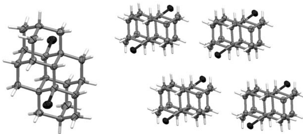
Figure 3. The X-ray structure of dibromide 24 and its crystal packing.
