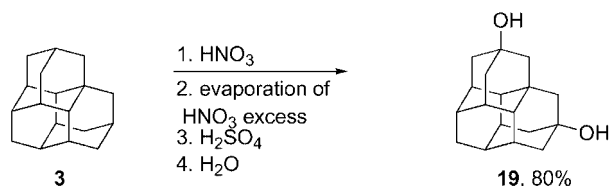
Scheme 6. One-pot preparation of bis-apical diol 19 from triamantane ( 3 ).
