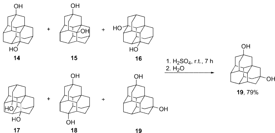
Scheme 5. Thermodynamically controlled isomerization of triamantane diols.
