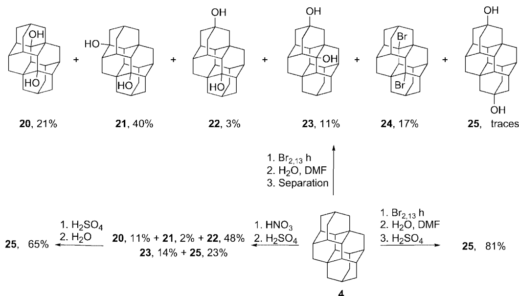
Scheme 7. Bis-functionalizations of [121]tetramantane ( 4 ).
