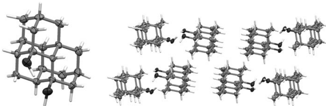
Figure 2. The X-ray structure (50% probability) of diol 17 and its crystal packing.
