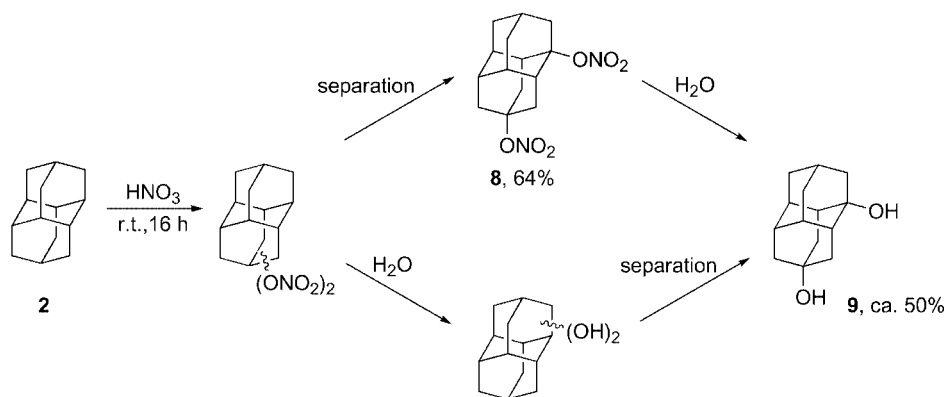
Scheme 2. Preparation of 1,4-dihydroxydiamantane ( 9 ) via nitroxylation and subsequent hydrolysis.
