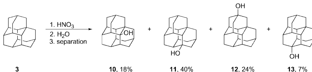
Scheme 3. Preparation of monohydroxy derivatives of triamantane ( 3 ).
