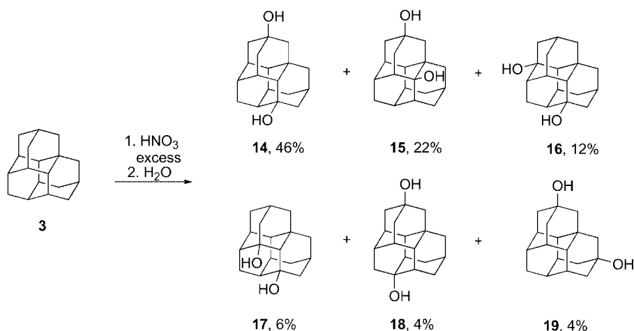
Scheme 4. Kinetically controlled bis-substitution of triamantane ( 3 ) with nitric acid.
