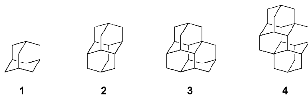
Figure 1. Diamondoids: adamantane (1), diamantane (2), triamantane (3), and [121]tetramantane (4).
