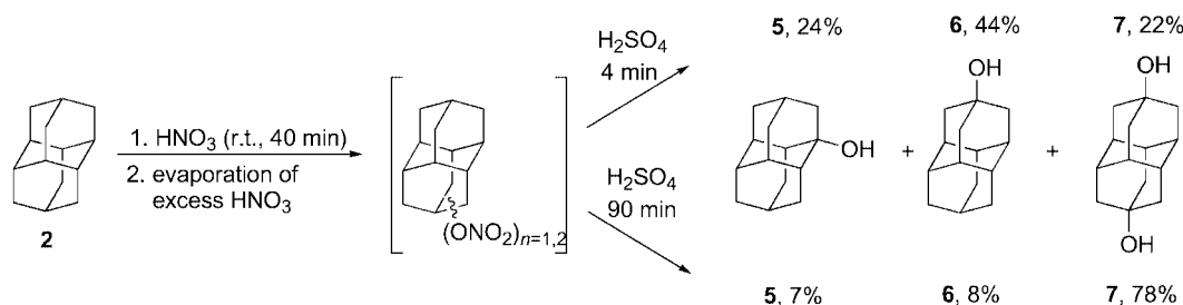
Scheme 1. Nitroxylation of diamantane (2) and subsequent isomerization (all yields are preparative).
